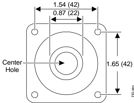
Mounting Flange Dimensions, in. (mm)
