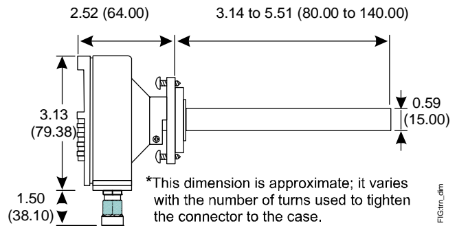
Transmitter Dimensions, in. (mm)
