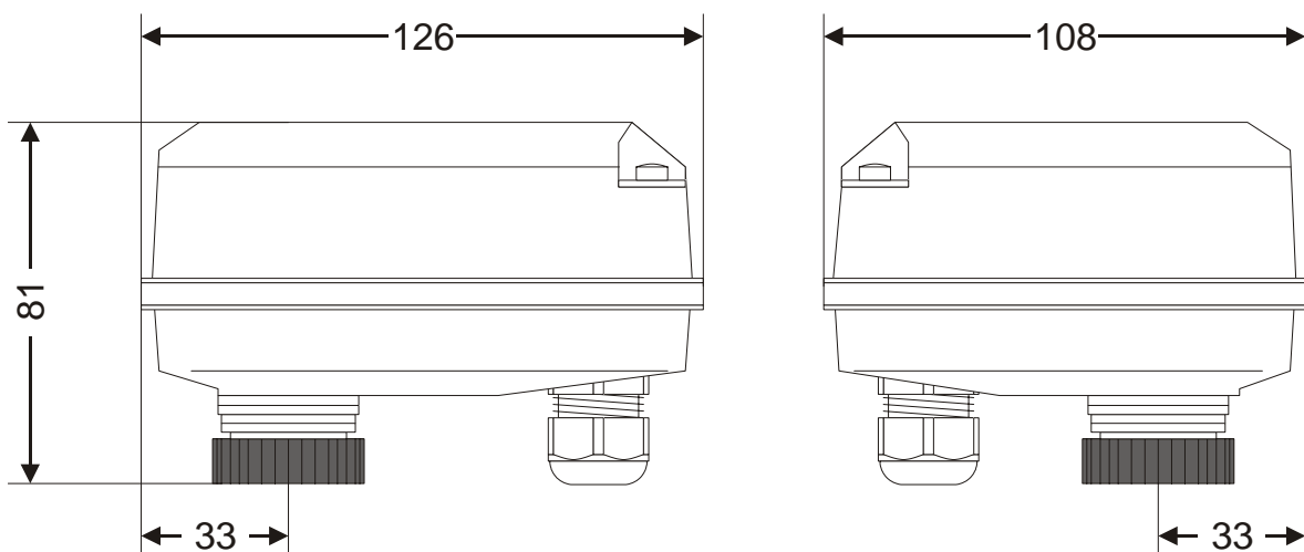
Fig. 3. ML7435E (dimensions in mm)
