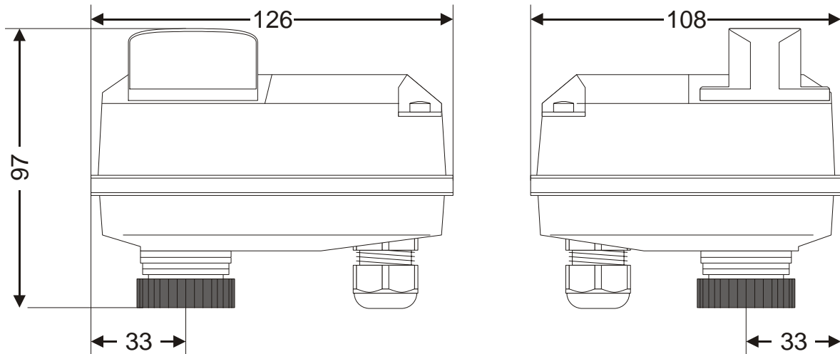
Fig. 2. ML7430E (dimensions in mm)
